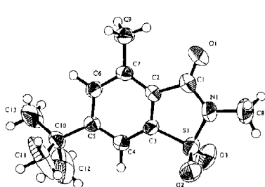
Fig. 1 X-Ray Crystal Structures of Compounds 2e-1 and 5e-1
