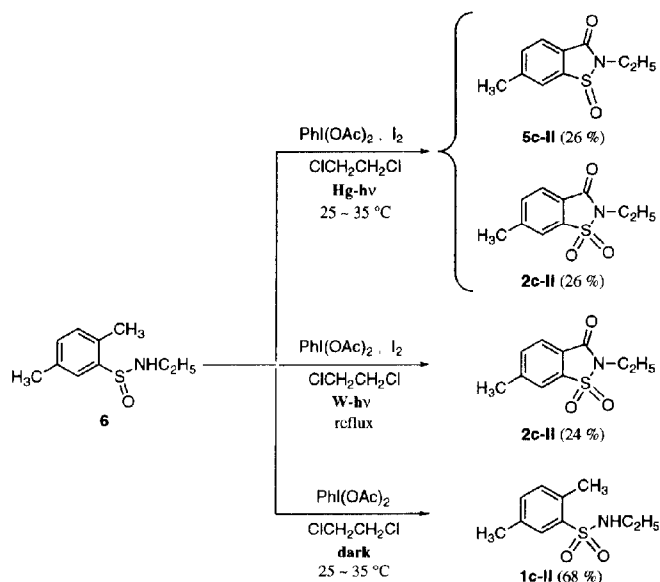
Scheme 2. Control Experiments
