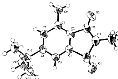
Fig. 1 X-Ray Crystal Structures of Compounds 2e-1 and 5e-1
