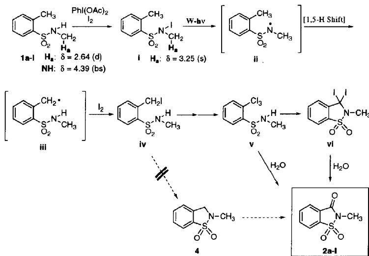
Scheme 1. Plausible Reaction Mechanism (Formation of 2a-I)
